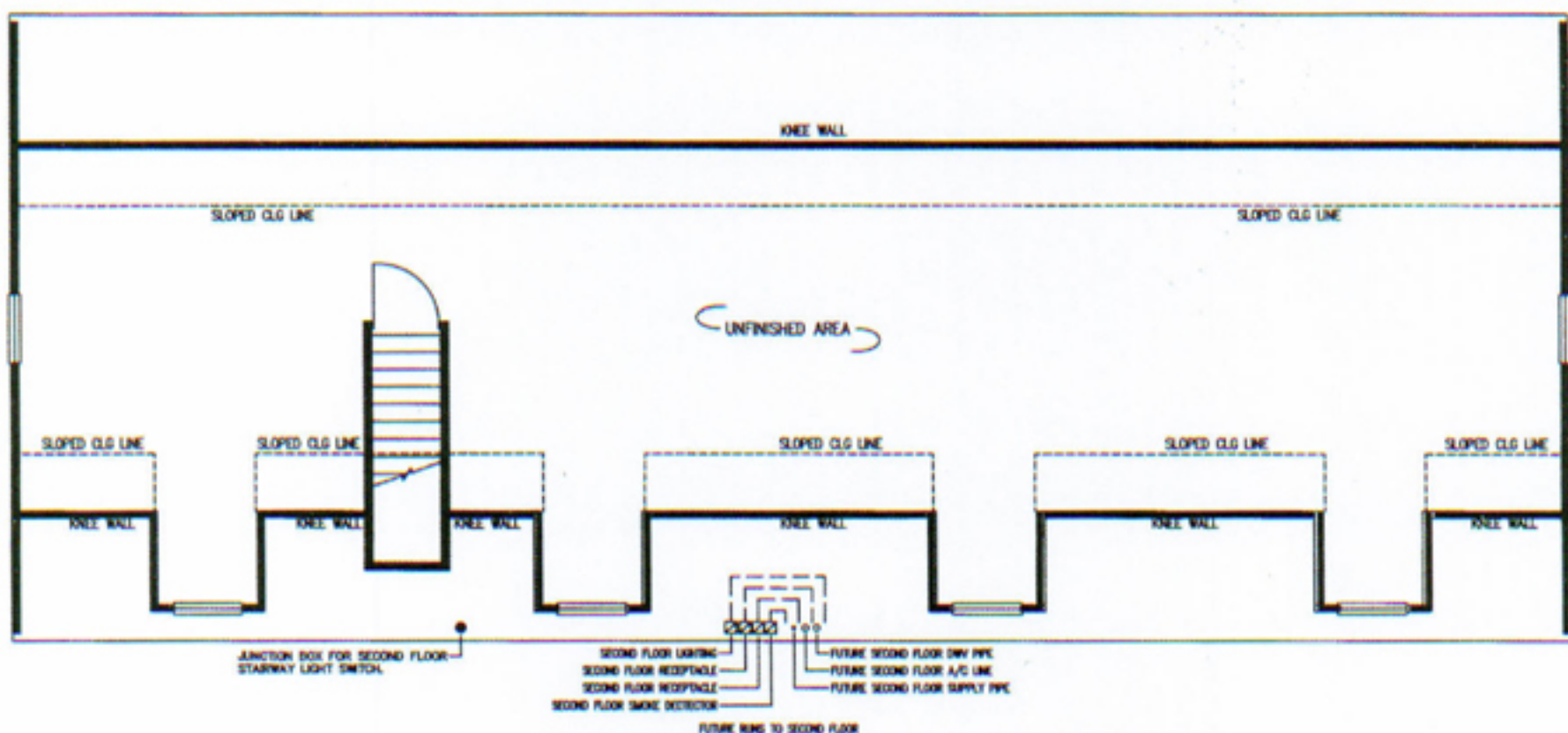
UNFINISHED SECOND FLOOR
